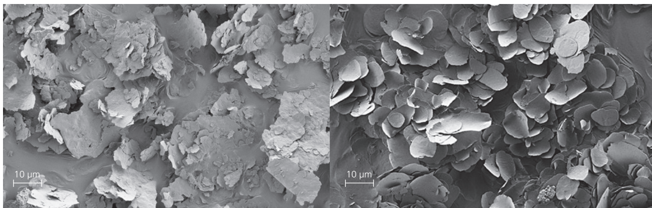
Microscopic pictures of PCS 1000 cornflake (left) in comparison to PCS 900 silverdollar (right) / Mikroskopische Bilder von PCS 1000 Cornflakes (links) und PCS 900 Silberdollar (rechts)
